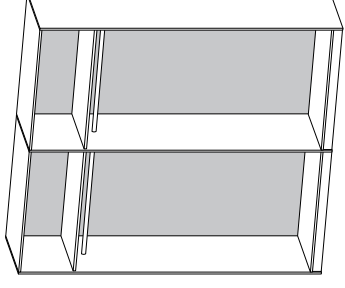
20001/68 Cabinet 195.5 x 58 x 199.4 cm 77 x 22.8 x 78.5"
